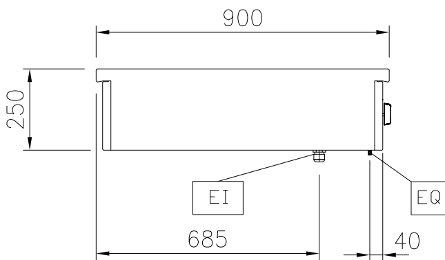
Lateral
